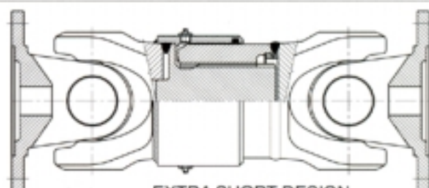
EXTRA SHORT DESIGN
