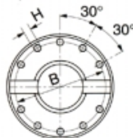
FLANGE WITH FACE KEY - STANDARD TYPE
