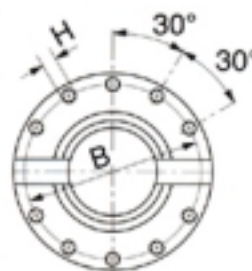
FLANGE WITH FACE KEY - STANDARD TYPE
