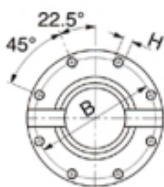
FLANGE WITH FACE KEY - STANDARD TYPE
