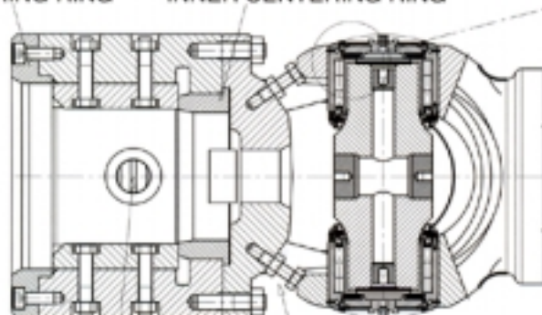
ROLL DETENT ASSEMBLY ANGLE LIMITERS
