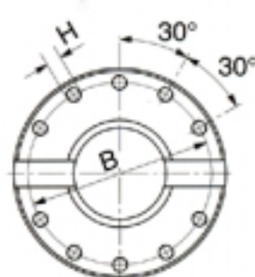
FLANGE WITH FACE KEY - LARGER TYPE
