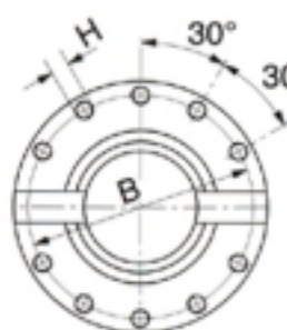
FLANGE WITH FACE KEY - LARGER TYPE
